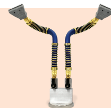
A Model 1122-9412 includes two Model 1122 Super Air Nozzles with two 12" (305mm) Stay Set Hose and Two Outlet Magnetic Base.
